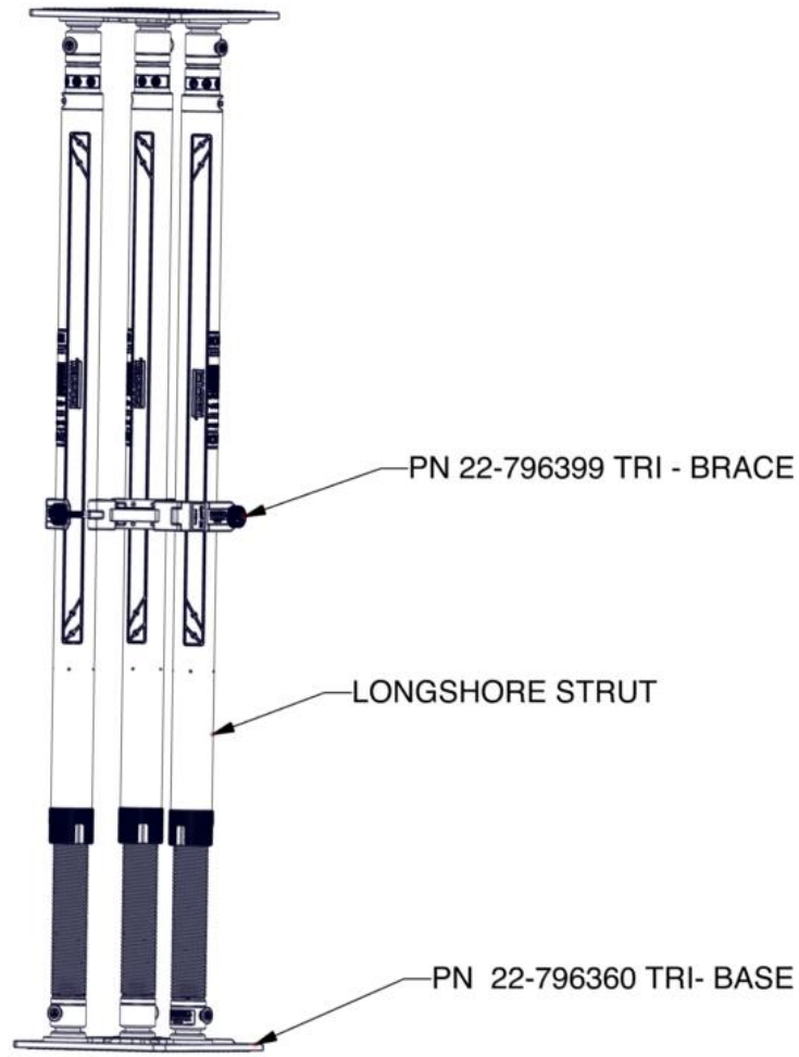
FRONT VIEW
